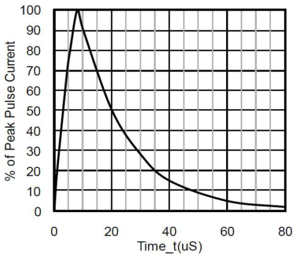
Figure 5. 8 X 20μs Pulse Waveform
