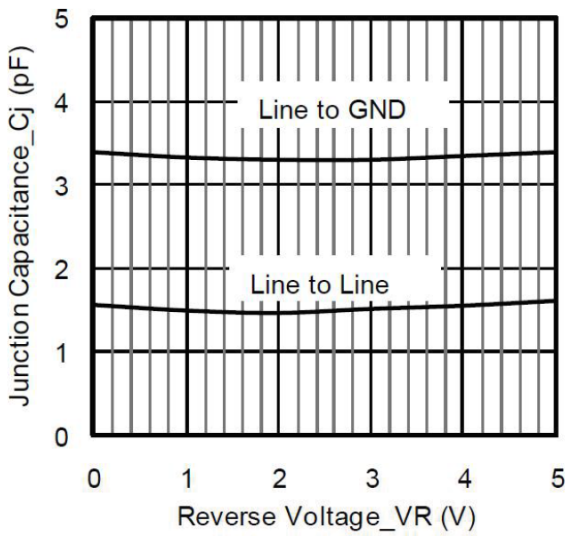
Figure 1. Junction Capacitance vs. Reverse Voltage
