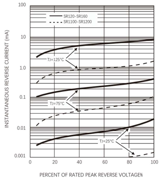
FIG.4-TYPICAL REVERSE CHARACTERISTICS
