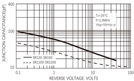
FIG.5-TYPICAL JUNCTION CAPACITANCE
