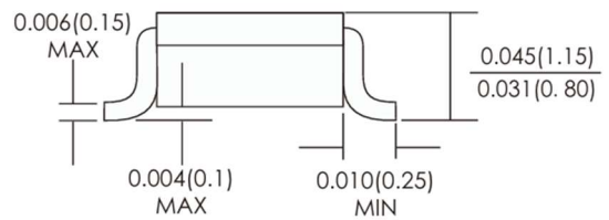
Dimensions in inches and (millimeters)
